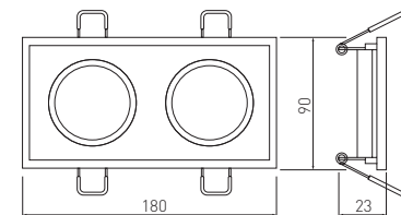
MR16 GZ-MR16-0000
