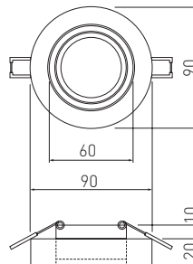
MR16 GZ-MR16-0000
