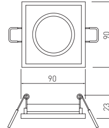
MR16 GZ-MR16-0000
