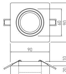
MR16 GZ-MR16-0000
