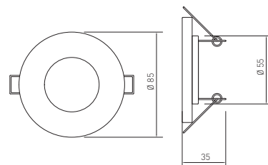
MR16 GZ-MR16-0000
